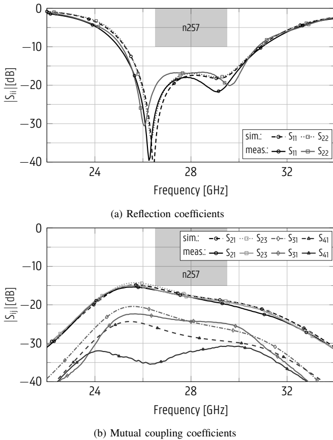
Fig. 9. Simulated and measured magnitude of the S-parameters of the 1×4 antenna array (SA-AA) referred to 50 Ω.
