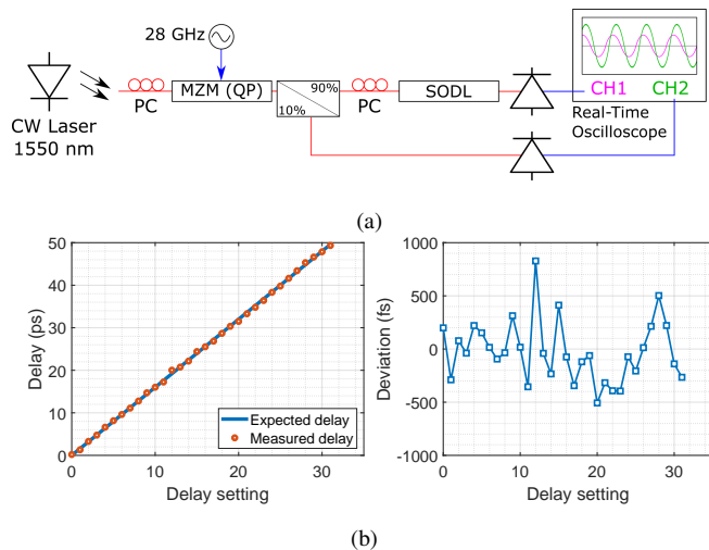
Fig. 11. Time delay performance of the proposed switched optical delay line (SODL). (a) Measurement setup (CW: continuous wave; MZM: Mach Zehnder Modulator; QP: Quadrature Point; PC: Polarization Controller). (b) Measured versus expected time delay and their corresponding deviation.
