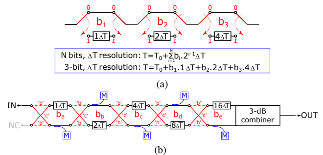
Fig. 2. Conceptual representation of a switchable optical delay line (SODL): (a) Standard 3-bit SODL. (b) Adopted 5-bit SODL to reduce number of control voltages. M: power monitor port; NC: not connected, 'b': bar state, 'c': cross state.
