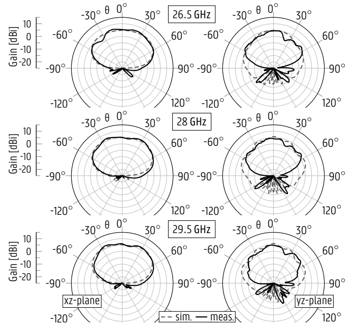
Fig. 10. Simulated and measured radiation pattern of the center element of the 1×4 antenna array (SA-AA).
