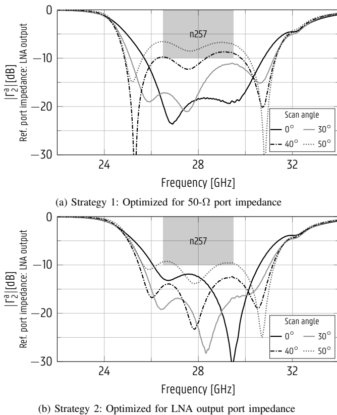
Fig. 7. Simulated magnitude of the active reflection coefficients of element 2 of both versions of the antenna array, when steering the beam to to \theta_0 = 0^\circ , 30^\circ , 40^\circ and 50^\circ . The reflection coefficients are referred to the conjugated LNA output impedance.
