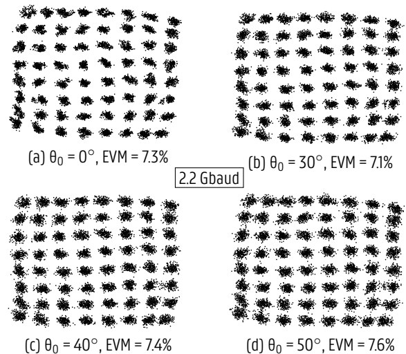
Fig. 14. Measured EVM of a 64-QAM wireless communication link between the proposed RAU and a WG-34 standard gain horn antenna when beamsteering to four distinct scan angles.
