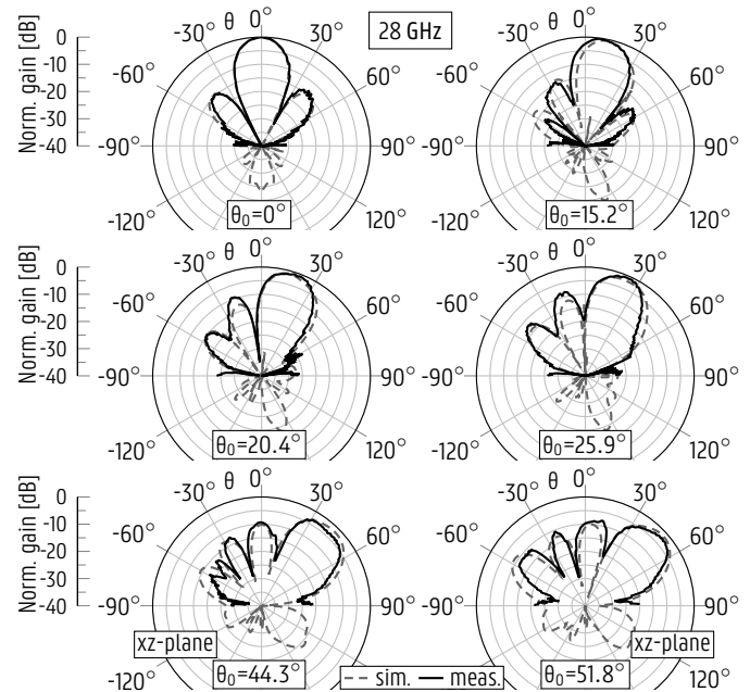
Fig. 13. Measured radiation pattern of the optically enabled beamforming RAU when the OBFN steers the beam to six distinct scan angles ( \theta_0 ). All the plots are normalized to the peak gain when beamsteering towards \theta_0 = 0^\circ .
