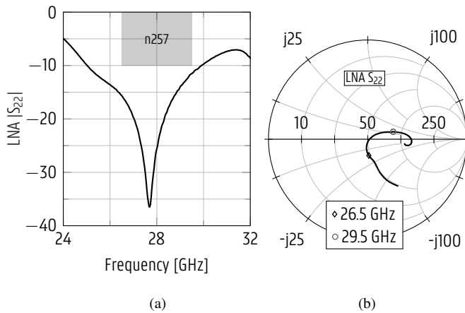
Fig. 6. Measured low-noise amplifier (LNA) output reflection coefficient: (a) Magnitude. (b) Smith chart.
